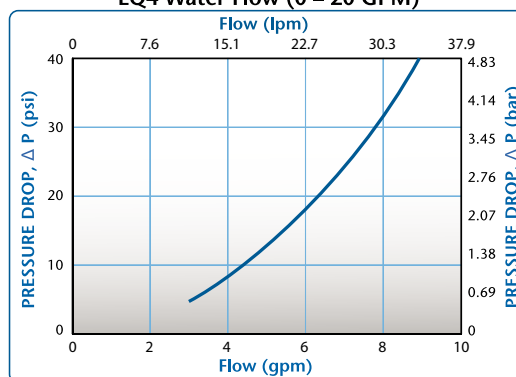
LQ4 Water Flow (0 – 20 GPM)
